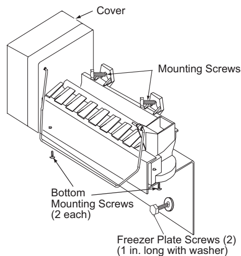
Figure 4. Mounting screws location.
