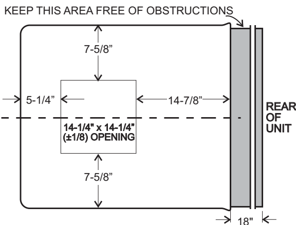
FIG. 1 AIR CONDITIONER/HEAT PUMP DIMENSIONS (On Top of Vehicle)
